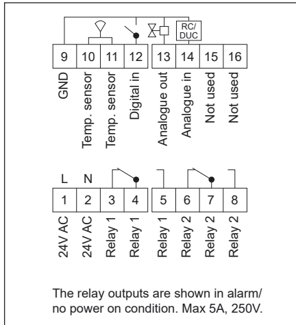
FIG. 2 (CFA-24V)
