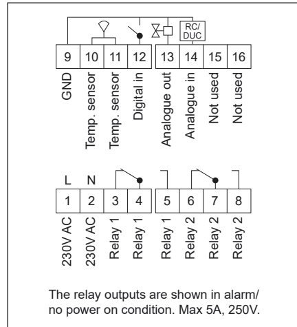
FIG. 3 (CFA-230V)
